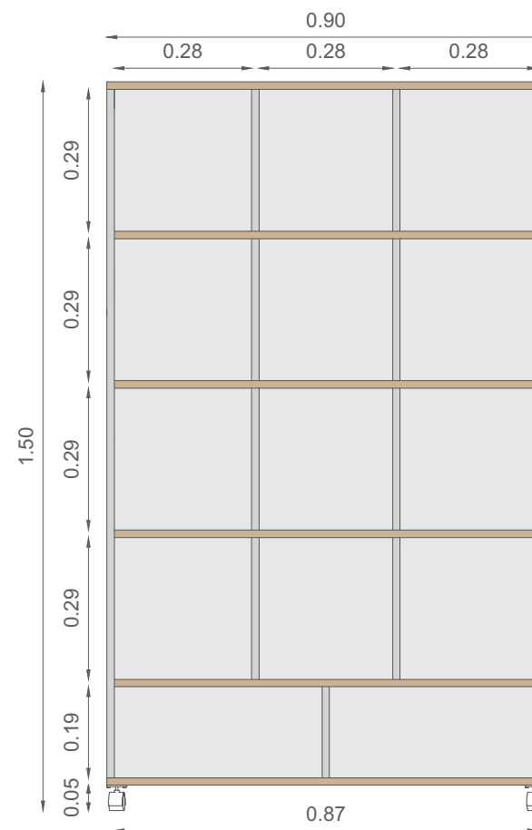
VISTA FRONTAL
